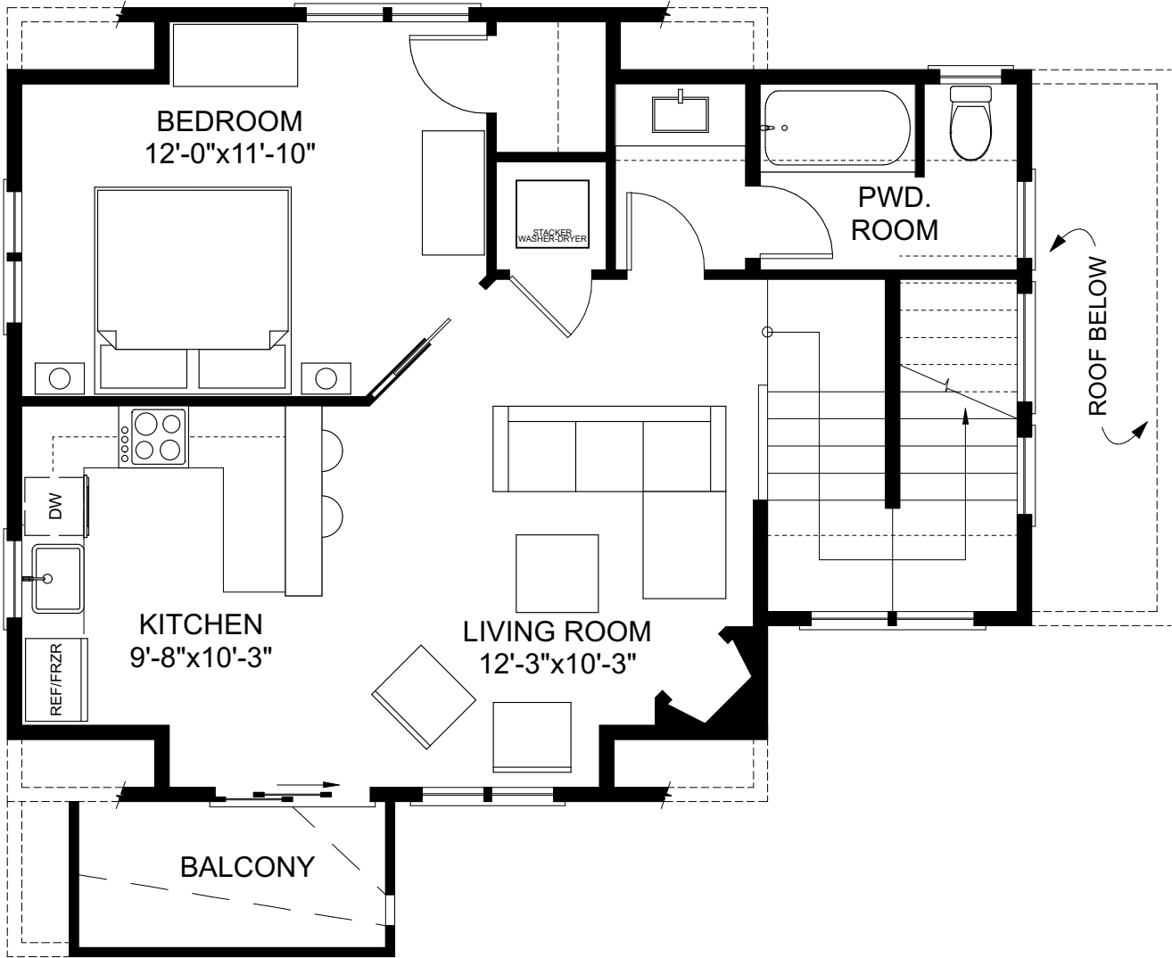
SECOND FLOOR
