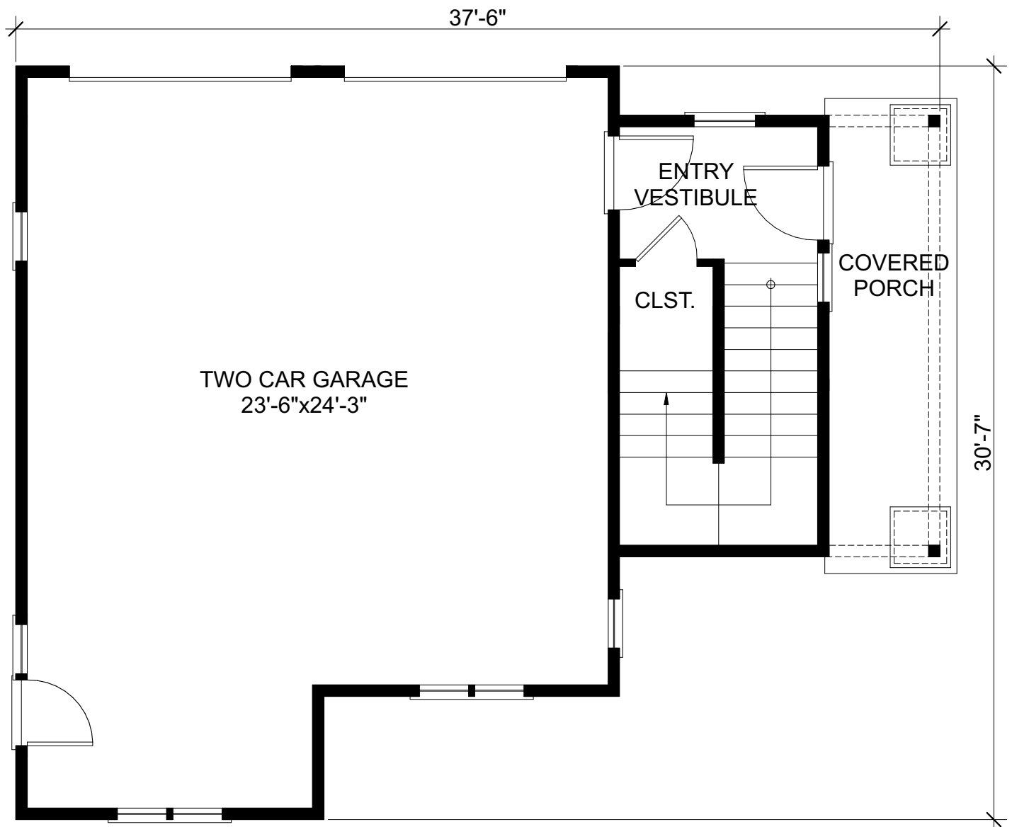
FIRST FLOOR
