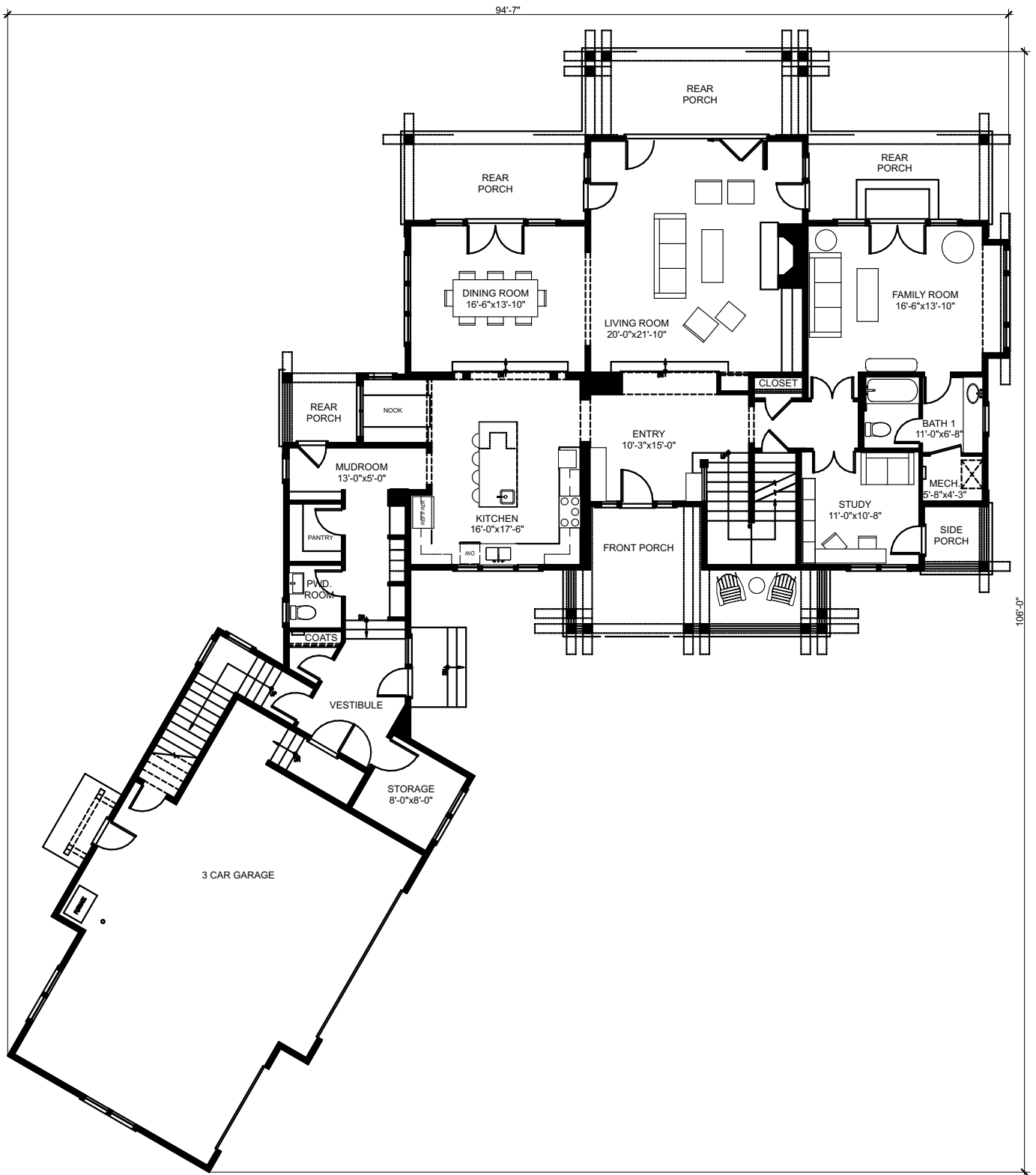
FIRST FLOOR
