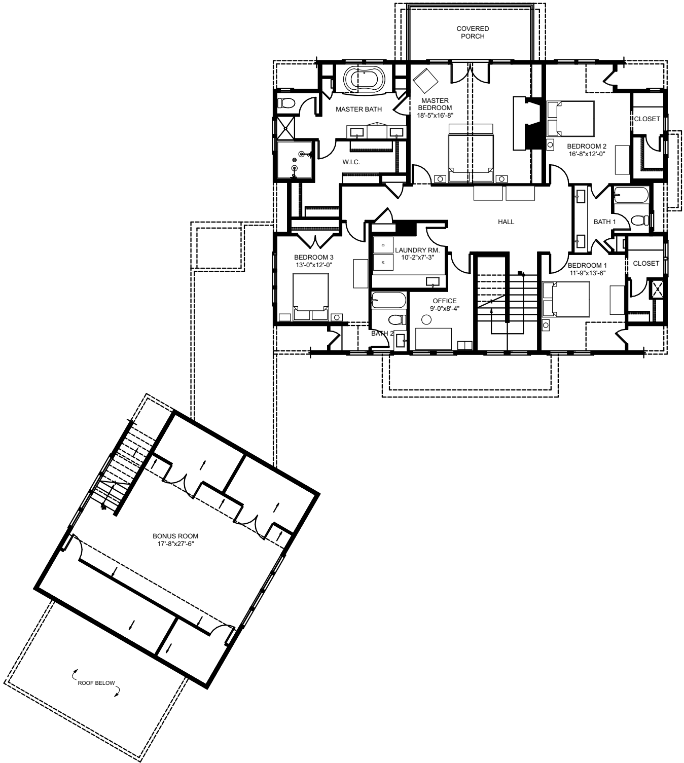
SECOND FLOOR
