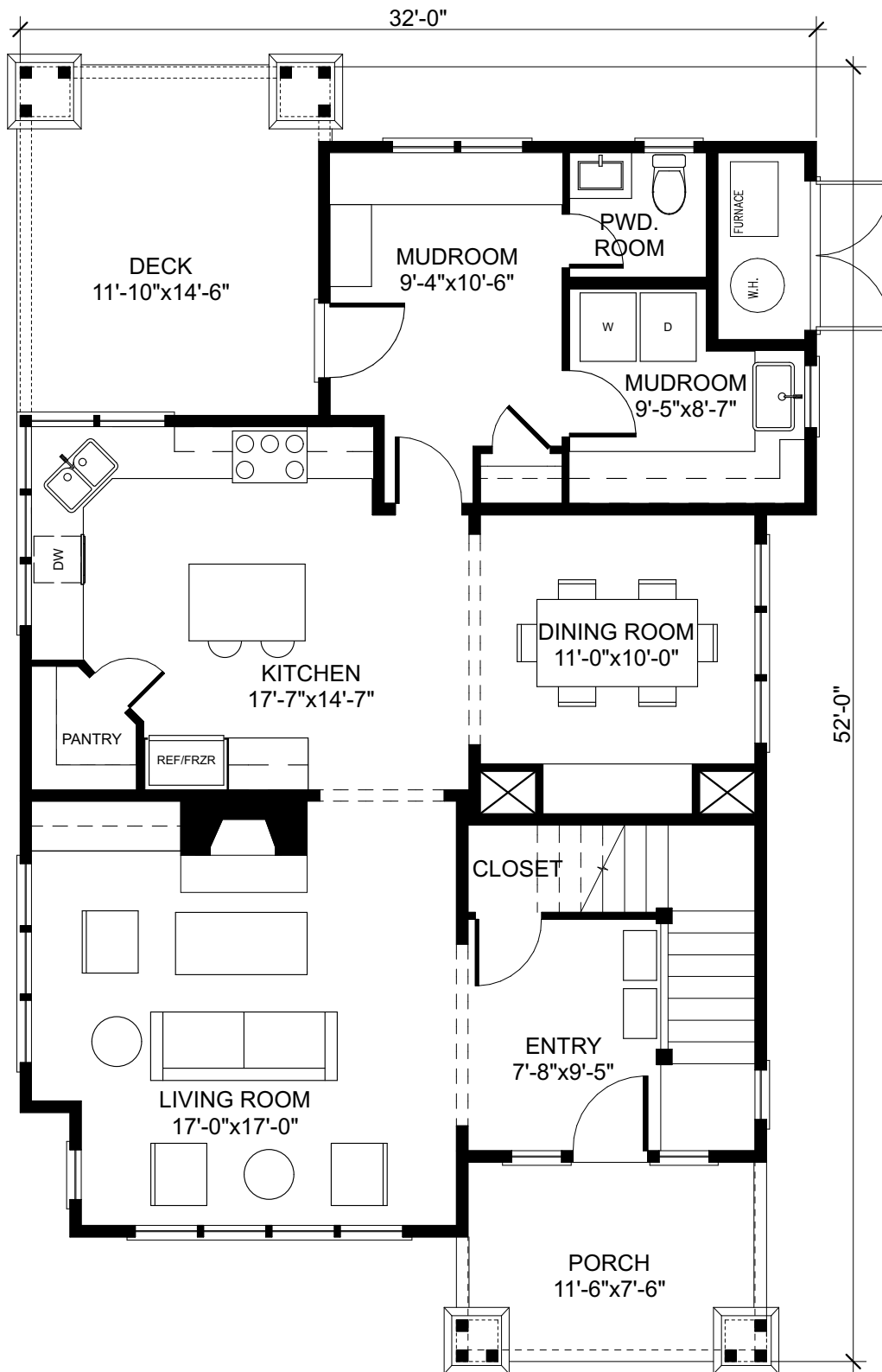
FIRST FLOOR
