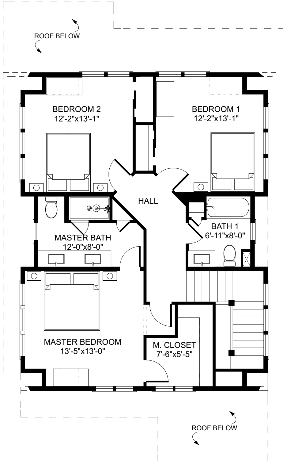
SECOND FLOOR
